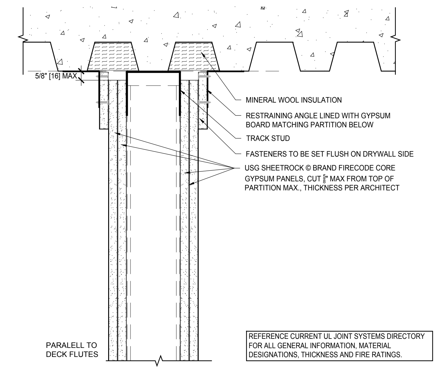
3 2 HR HEAD OF WALL UL HW-D-0002 Scale: 3" = 1' - 0"
