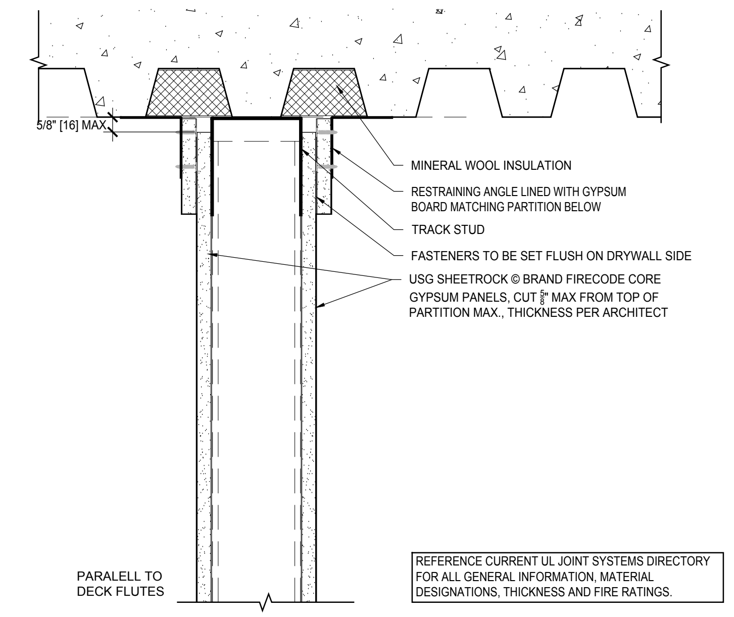
2 1 HR HEAD OF WALL UL HW-D-0001 Scale: 3" = 1' - 0"
