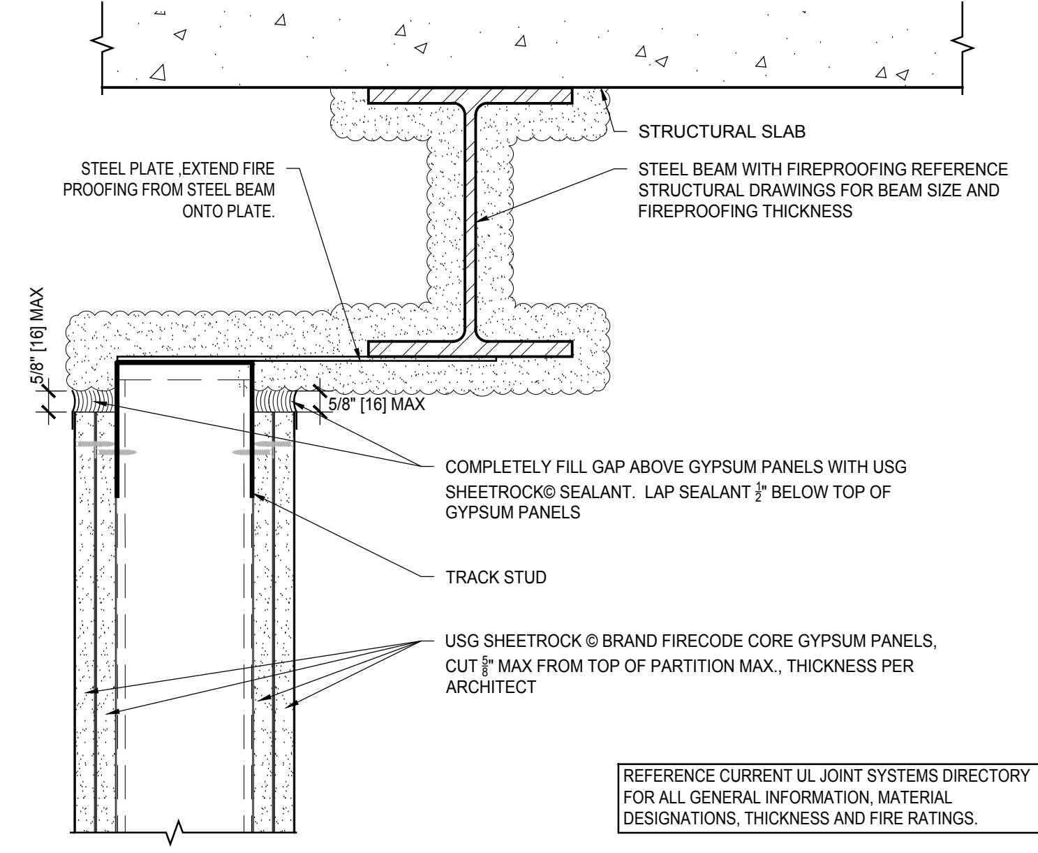
2 2 HR HEAD OF WALL UL HW-D-0628 Scale: 3" = 1' - 0"
