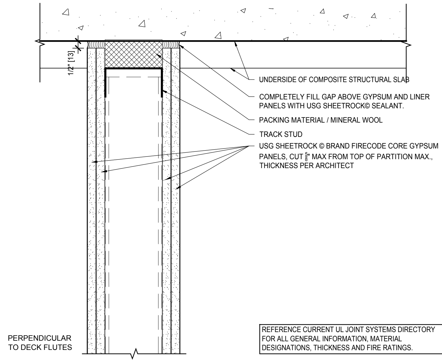
7 2 HR HEAD OF WALL UL HW-S-0035 Scale: 3" = 1' - 0"
