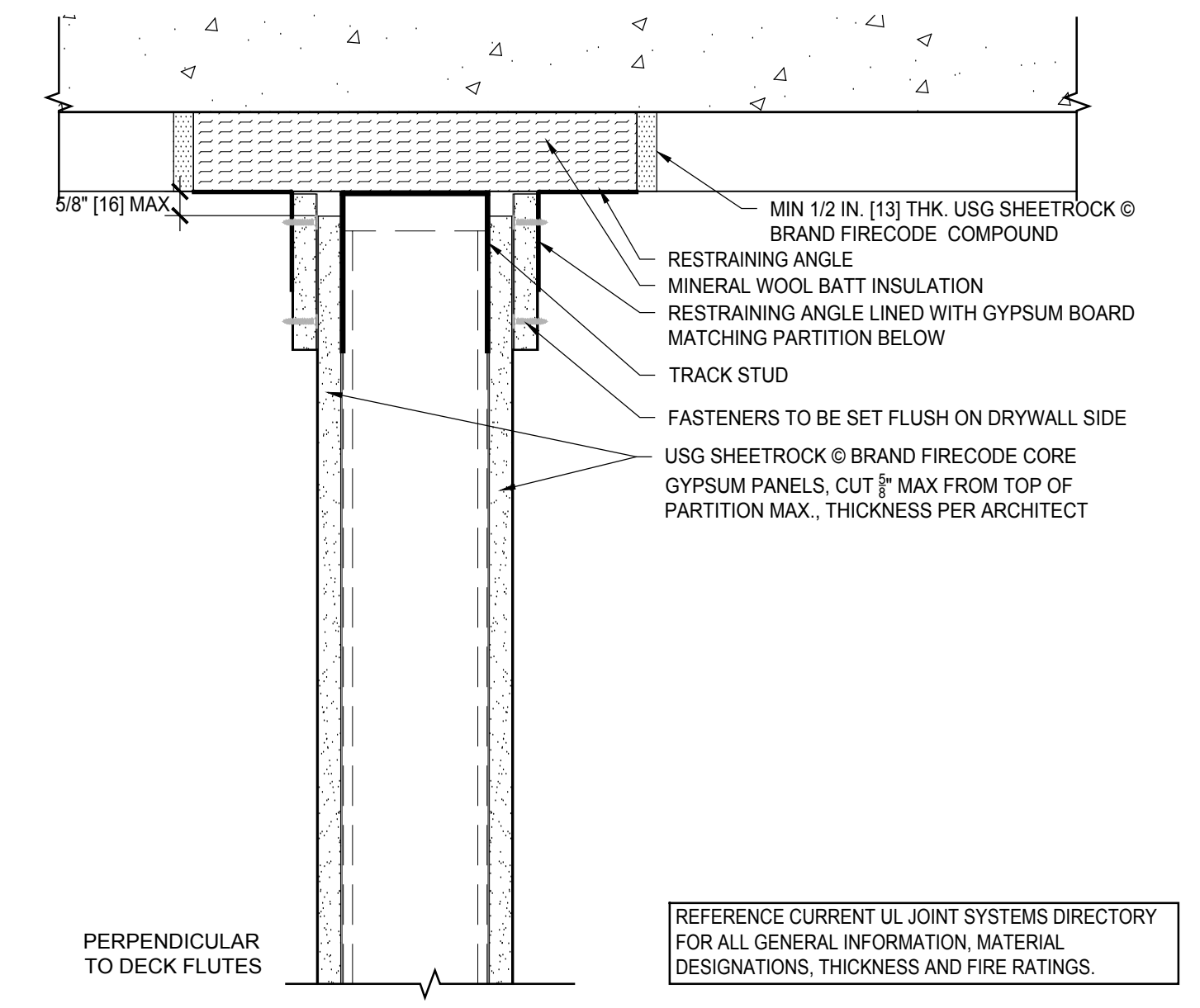
5 1 HR HEAD OF WALL UL HW-D-0001 Scale: 3" = 1' - 0"
