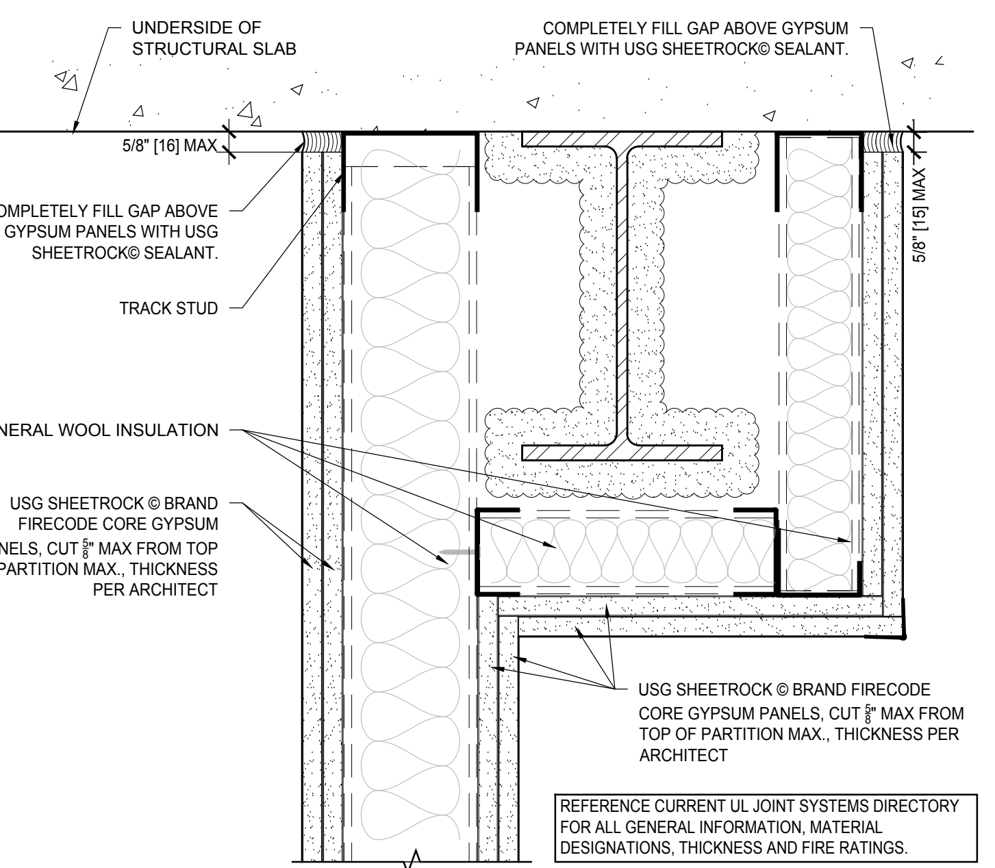
4 2 HR HEAD OF WALL AT BEAM Scale: 3" = 1' - 0"
