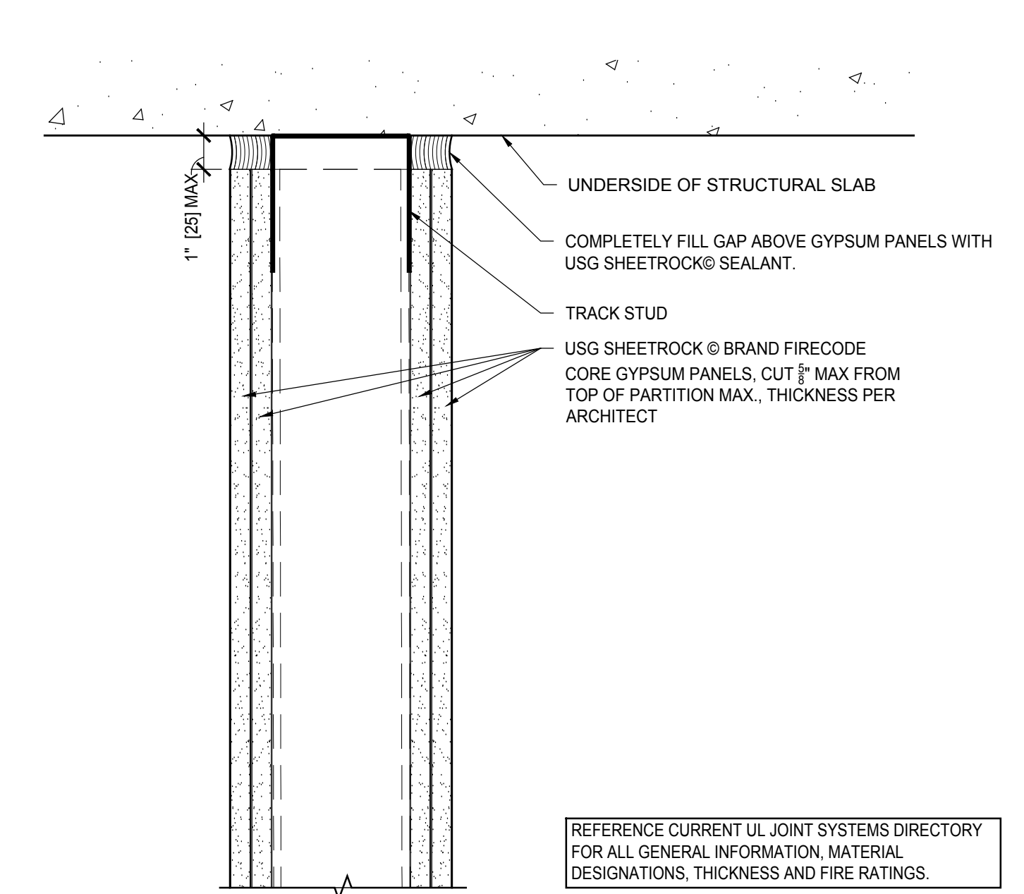
7 2 HR HEAD OF WALL UL HW-D-0158 Scale: 3" = 1' - 0"
