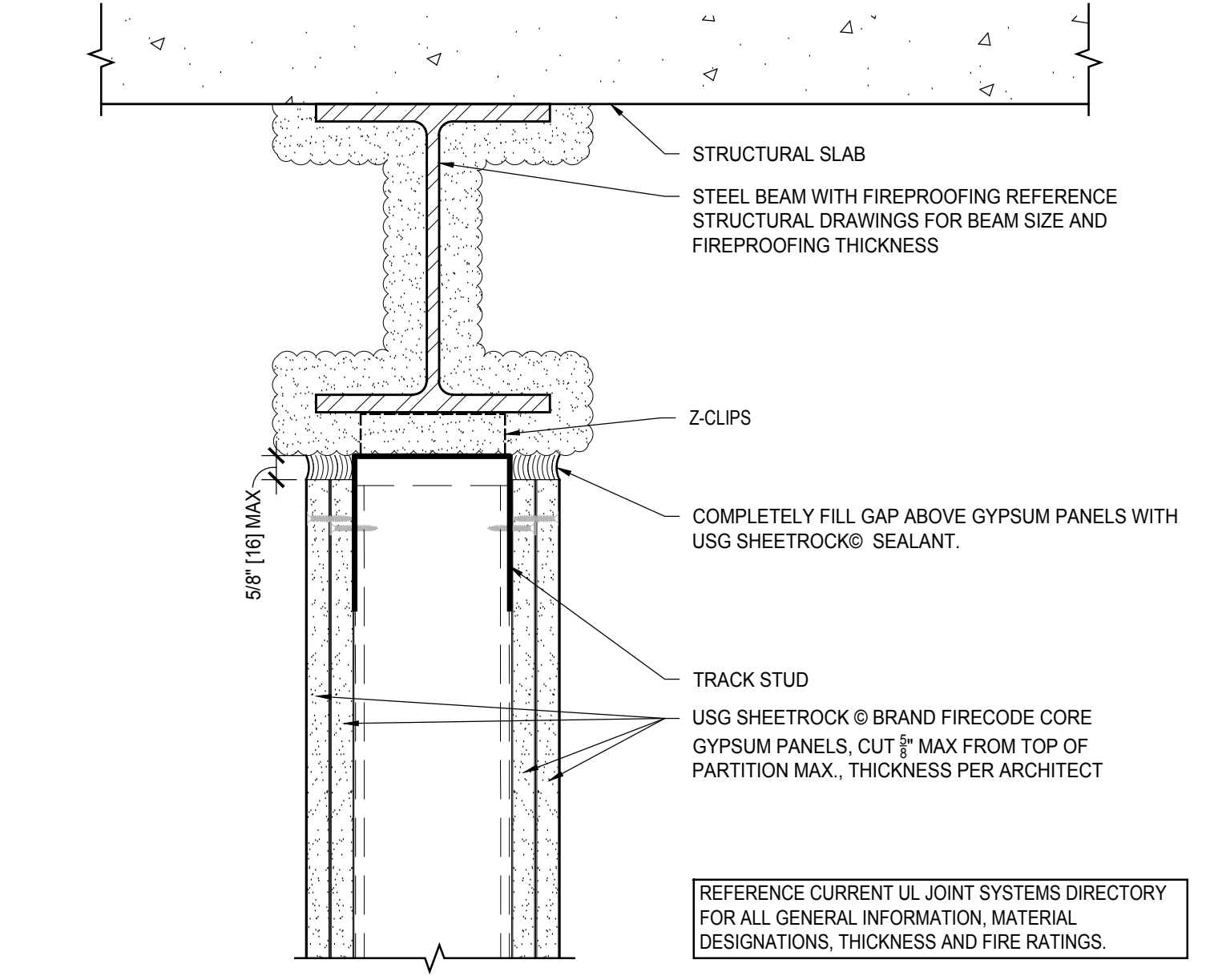
12 2 HR HEAD OF WALL UL HW-D-0626 Scale: 3" = 1' - 0"
