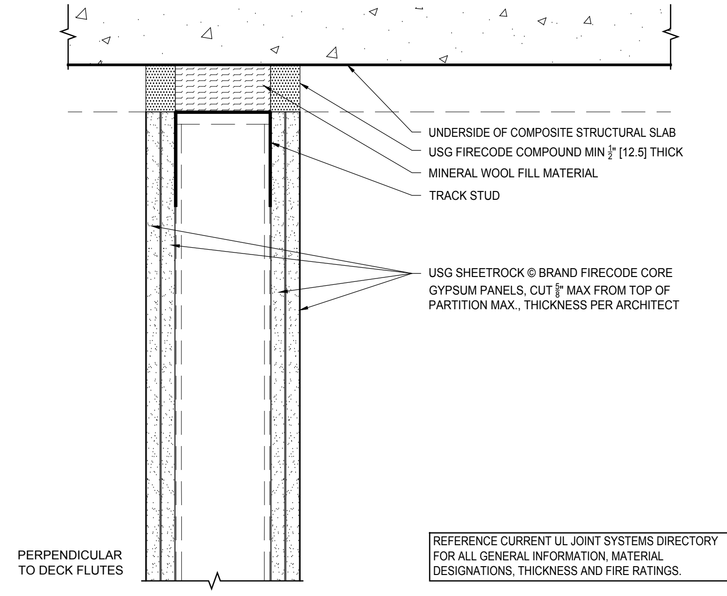
4 2 HR HEAD OF WALL UL HW-S-0001 Scale: 3" = 1' - 0"
