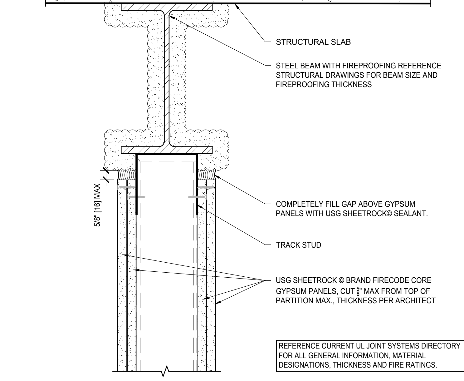
1 2 HR HEAD OF WALL UL HW-D-0627 Scale: 3" = 1' - 0"
