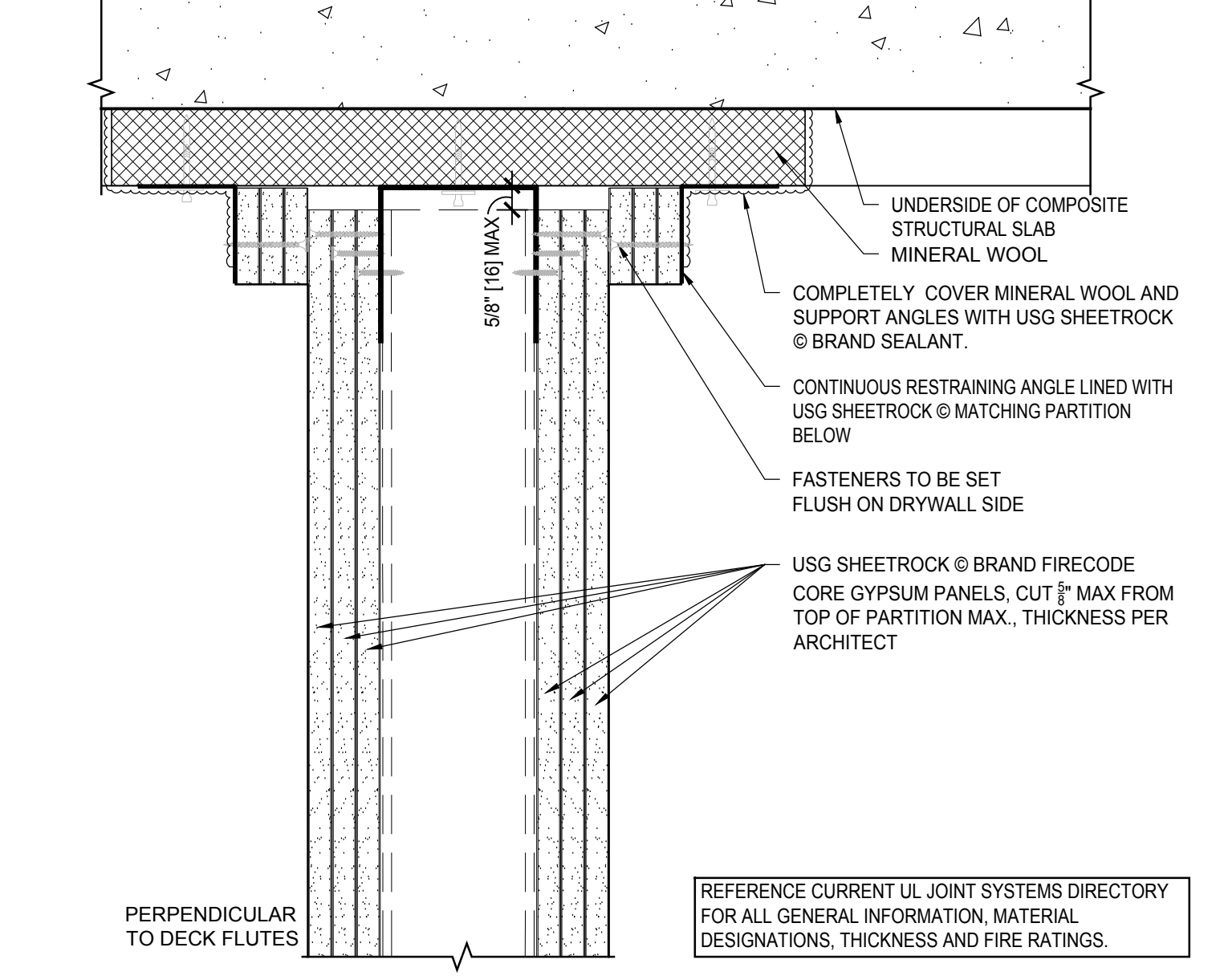
11 3 HR HEAD OF WALL UL HW-D-0614 Scale: 3" = 1' - 0"
