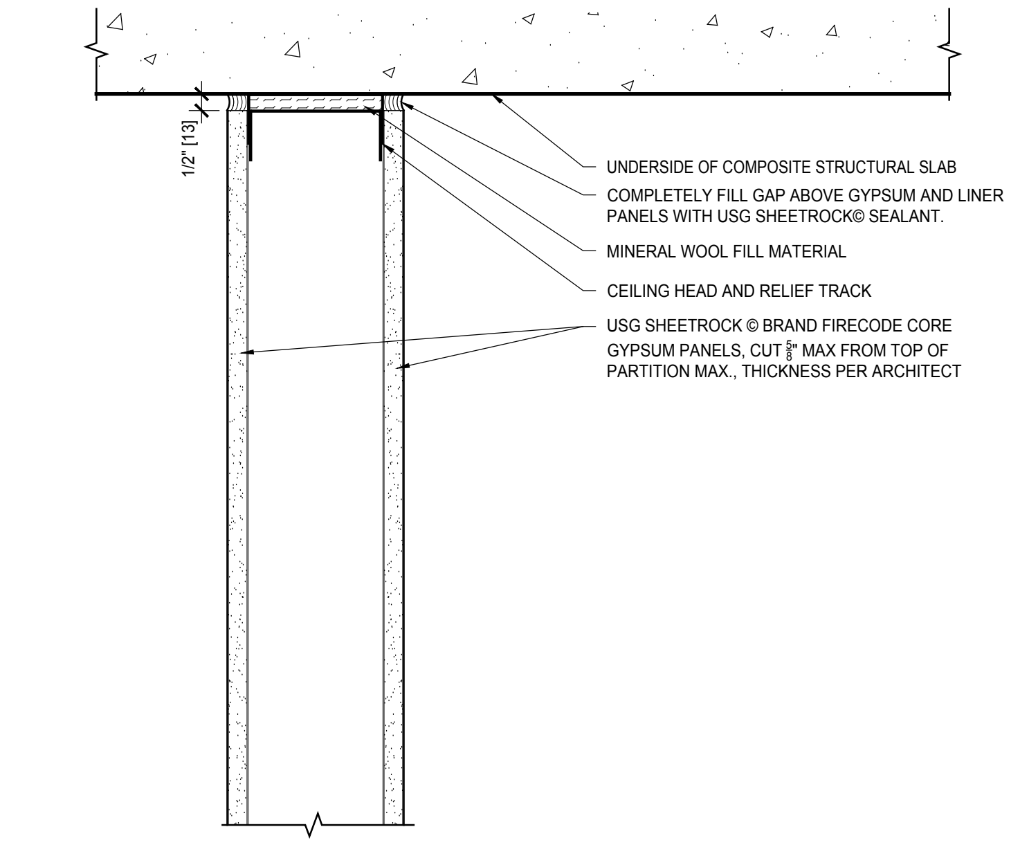
5 1 HR HEAD OF WALL UL HW-S-0009 Scale: 3" = 1' - 0"
