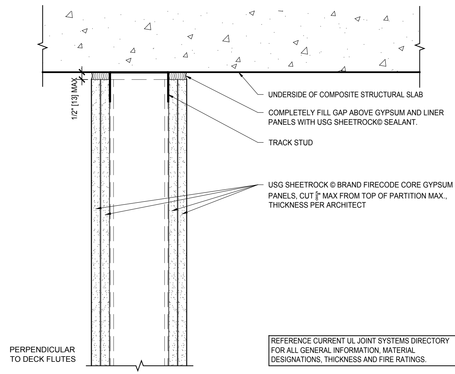
6 2 HR HEAD OF WALL UL HW-S-0032 Scale: 3" = 1' - 0"
