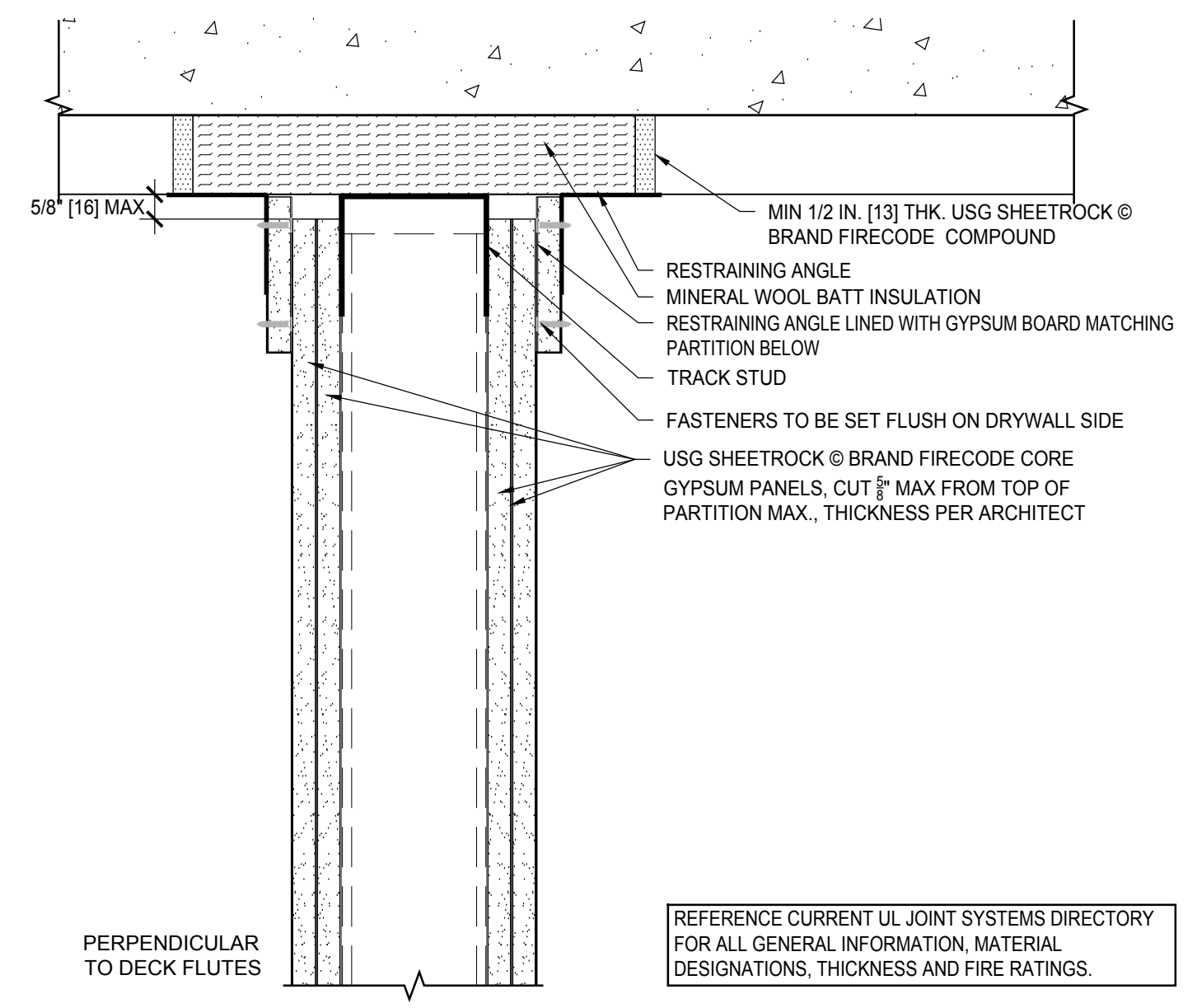
6 2 HR HEAD OF WALL UL HW-D-0002 Scale: 3" = 1' - 0"
