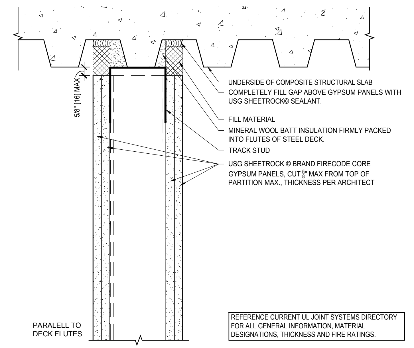
9 2 HR HEAD OF WALL UL HW-D-0262 Scale: 3" = 1' - 0"
