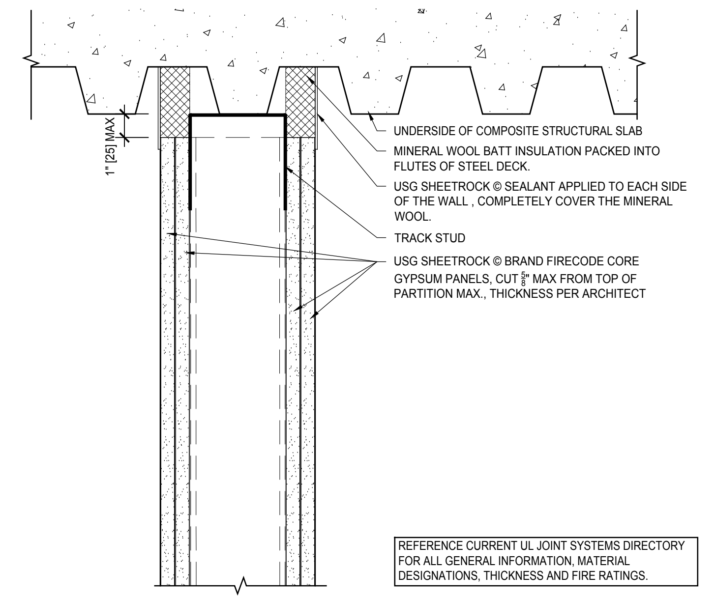
8 2 HR Head OF WALL UL HW-D-0160 Scale: 3" = 1' - 0"
