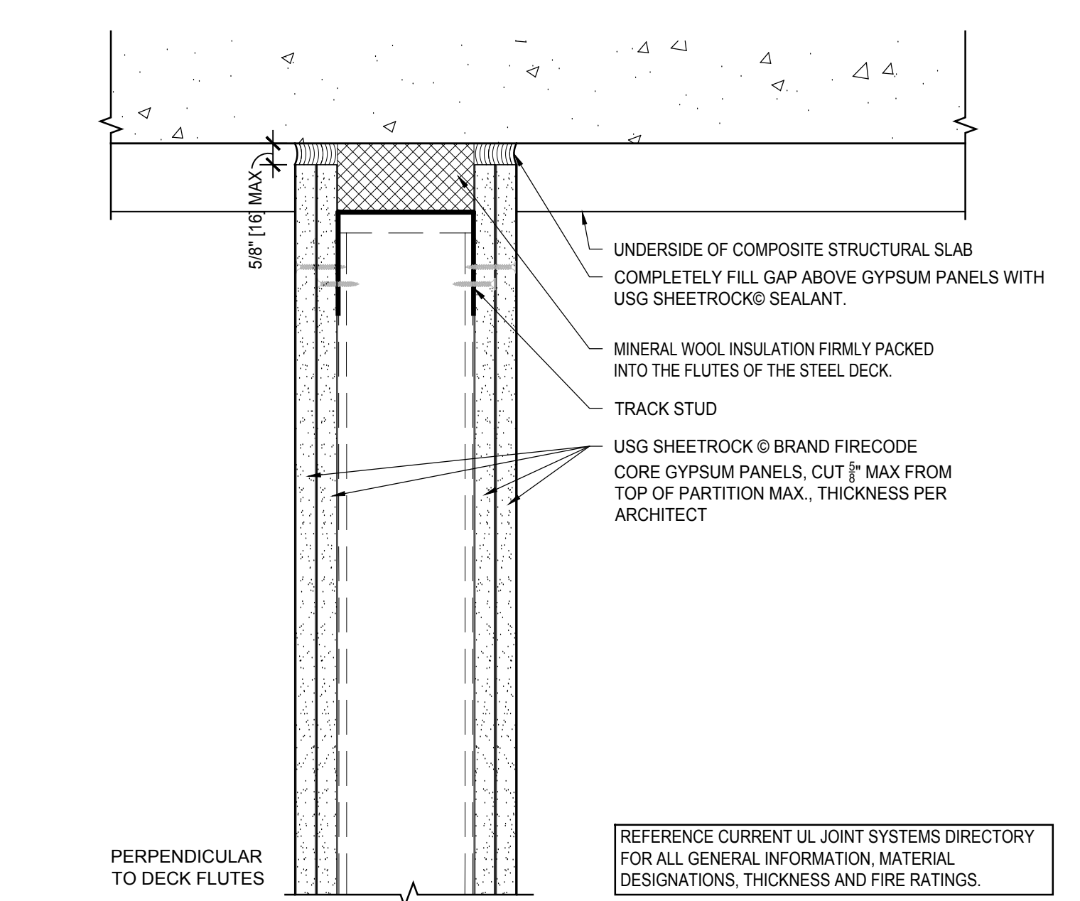
10 2 HR HEAD OF WALL UL HW-D-0262 Scale: 3" = 1' - 0"
