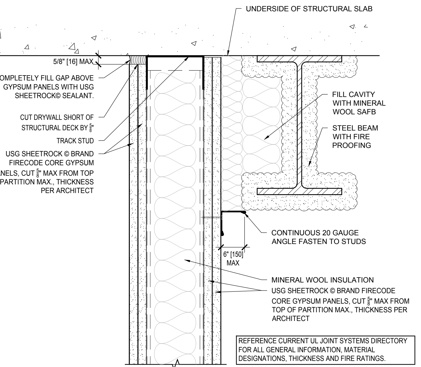
1 2 HR HEAD OF WALL ADJACENT TO BEAM Scale: 3" = 1' - 0"
