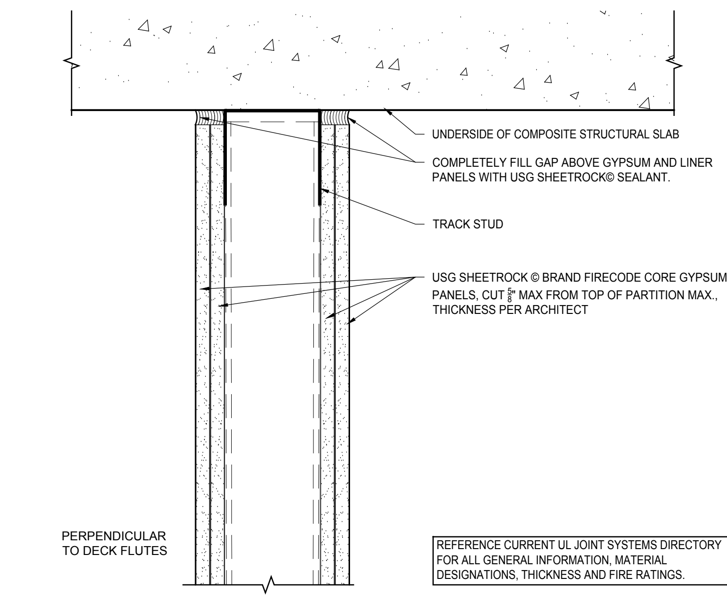
3 2 HR HEAD OF WALL UL HW-D-0632 Scale: 3" = 1' - 0"
