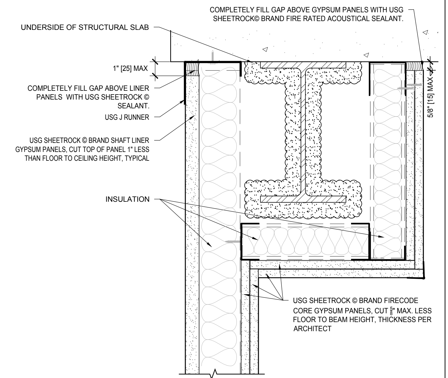
3 2 HR HEAD OF WALL ADJACENT TO BEAM Scale: 3" = 1' - 0"
