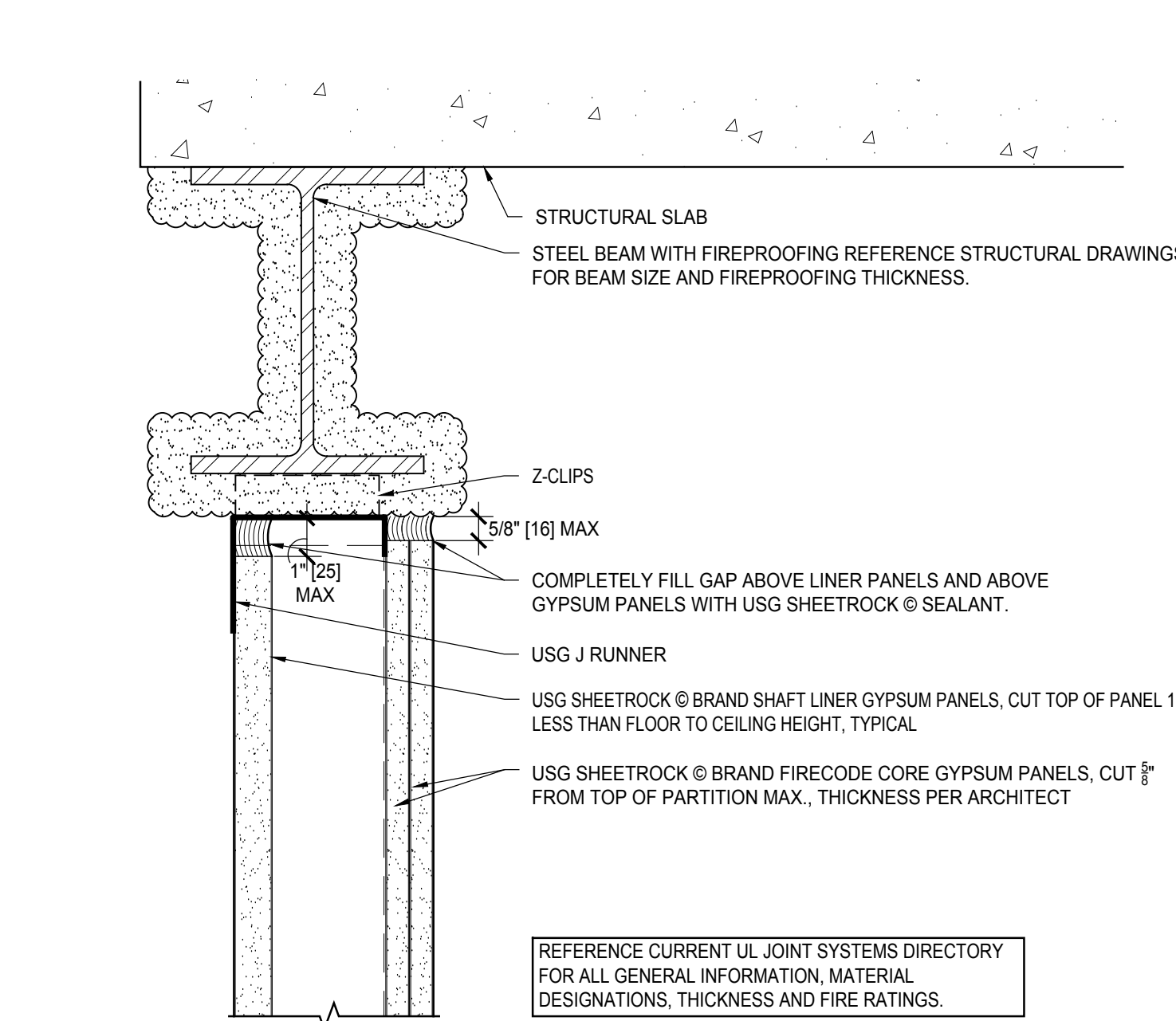
5 HEAD OF WALL UL HW-D-0609 (1 AND 2 HOUR) Scale: 3" = 1' - 0"
