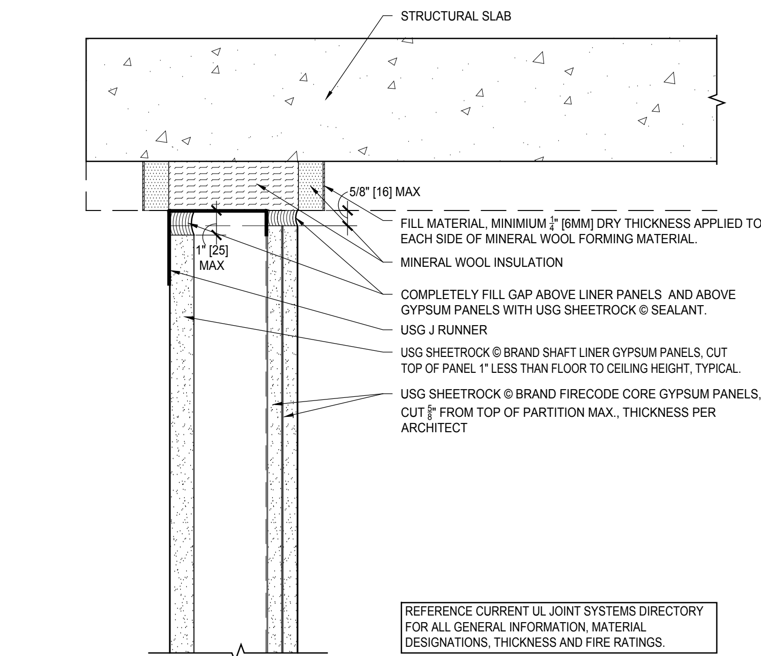
8 HEAD OF WALL UL HW-D-0612 (1 AND 2 HOUR) Scale: 3" = 1' - 0"
