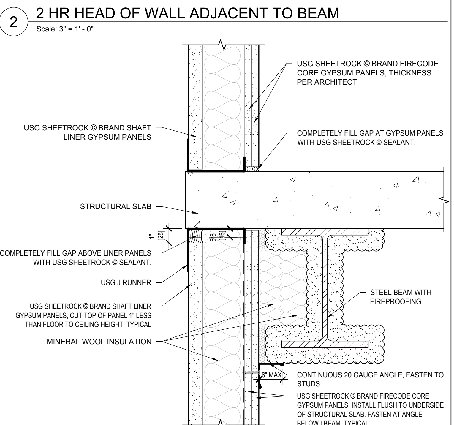
1 2 HR SHAFTWALL ADJACENT TO BEAM Scale: 3" = 1' - 0"
