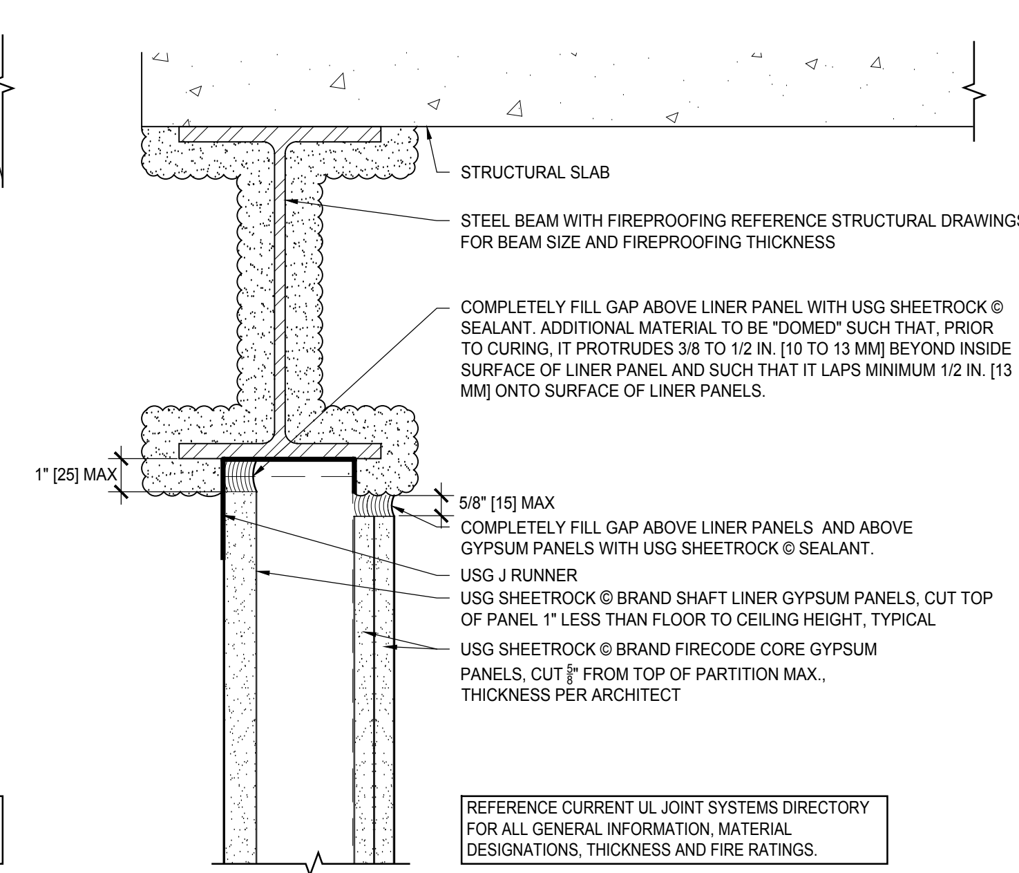
6 HEAD OF WALL UL HW-D-0610 (1 AND 2 HOUR) Scale: 3" = 1' - 0"
