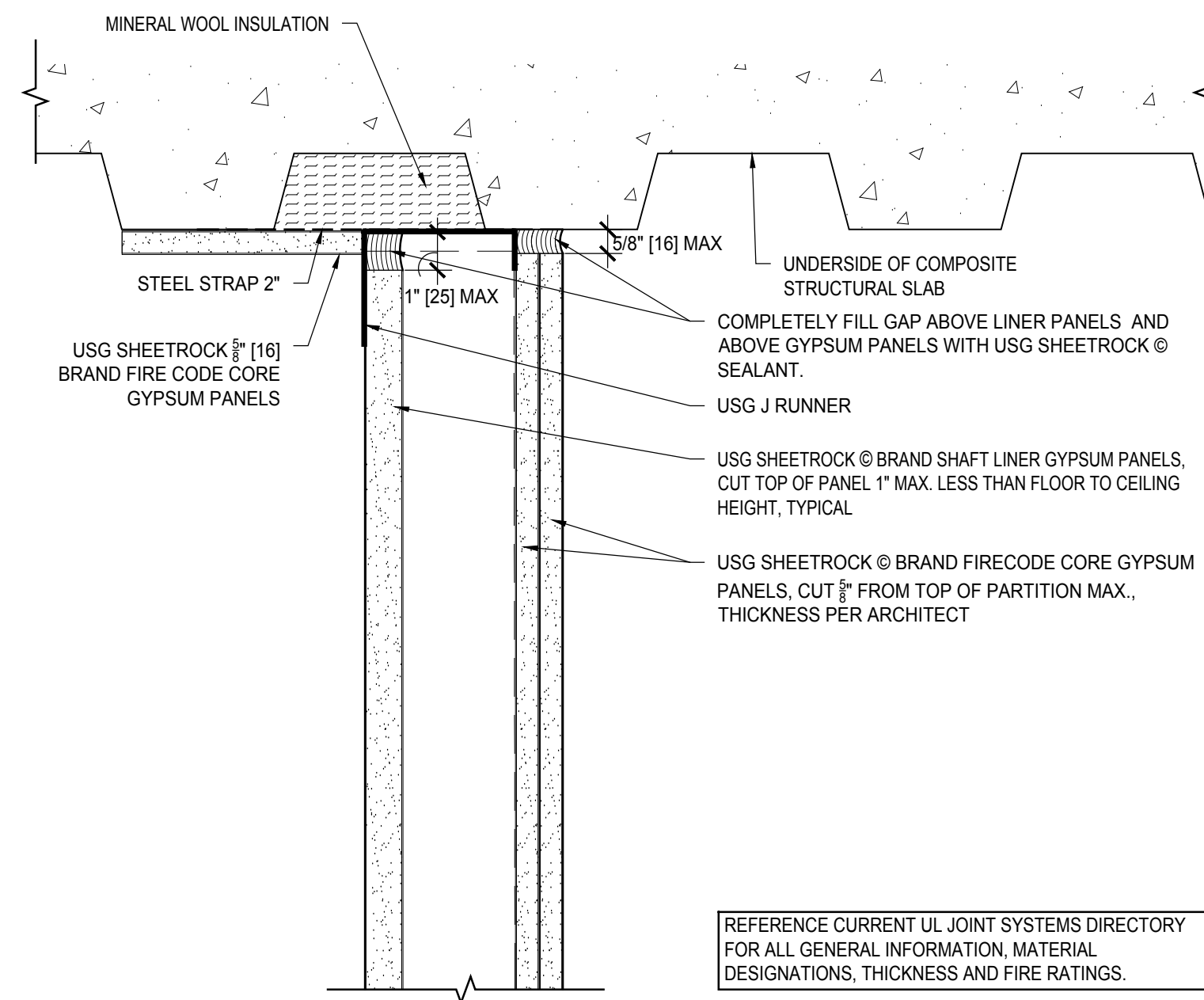
9 2 HR Head of Wall UL HW-D-0613 Scale: 3" = 1' - 0"
