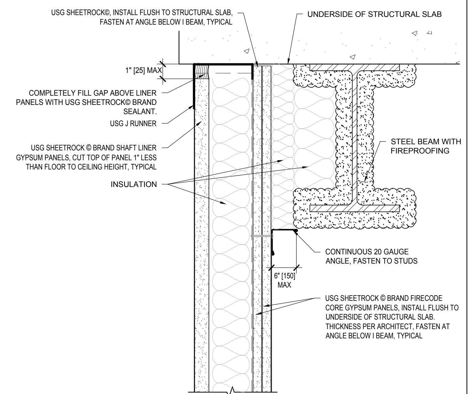
2 2 HR HEAD OF WALL ADJACENT TO BEAM Scale: 3" = 1' - 0"
