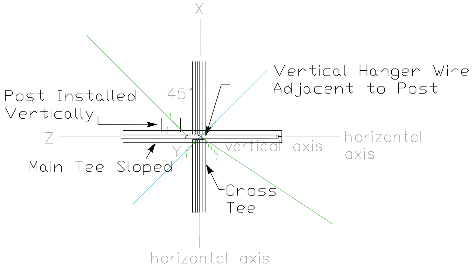
Top View (with splay wires at 45° from horizontal axes)
