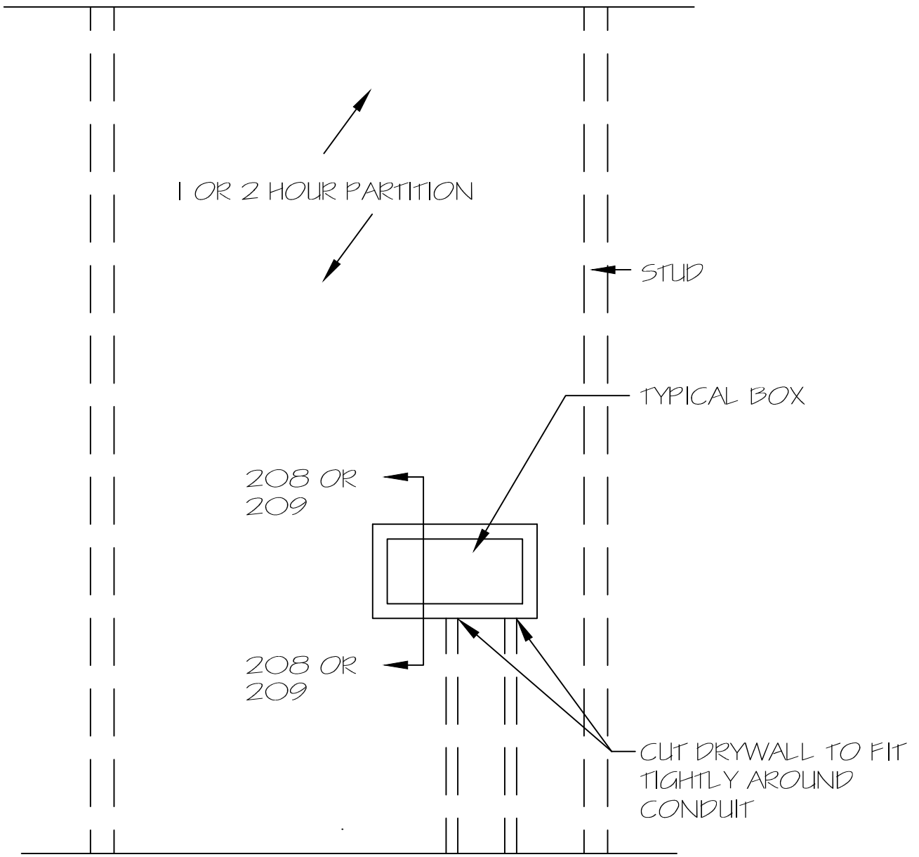
PARTIAL ELEVATION
